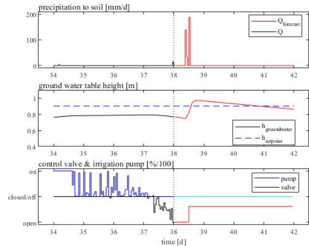
Fig 3. On-line snapshot of MPC in action at day 38. Past irrigation has changed to drainage, due to forecasted rain in the prediction horizon.
